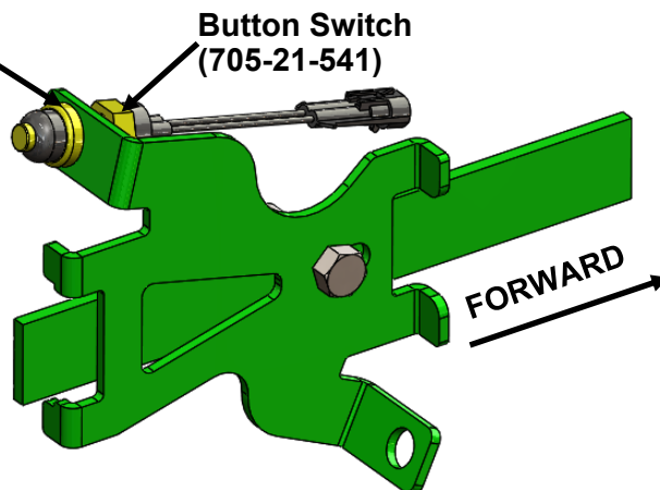
Long Linkage Bracket Configuration
